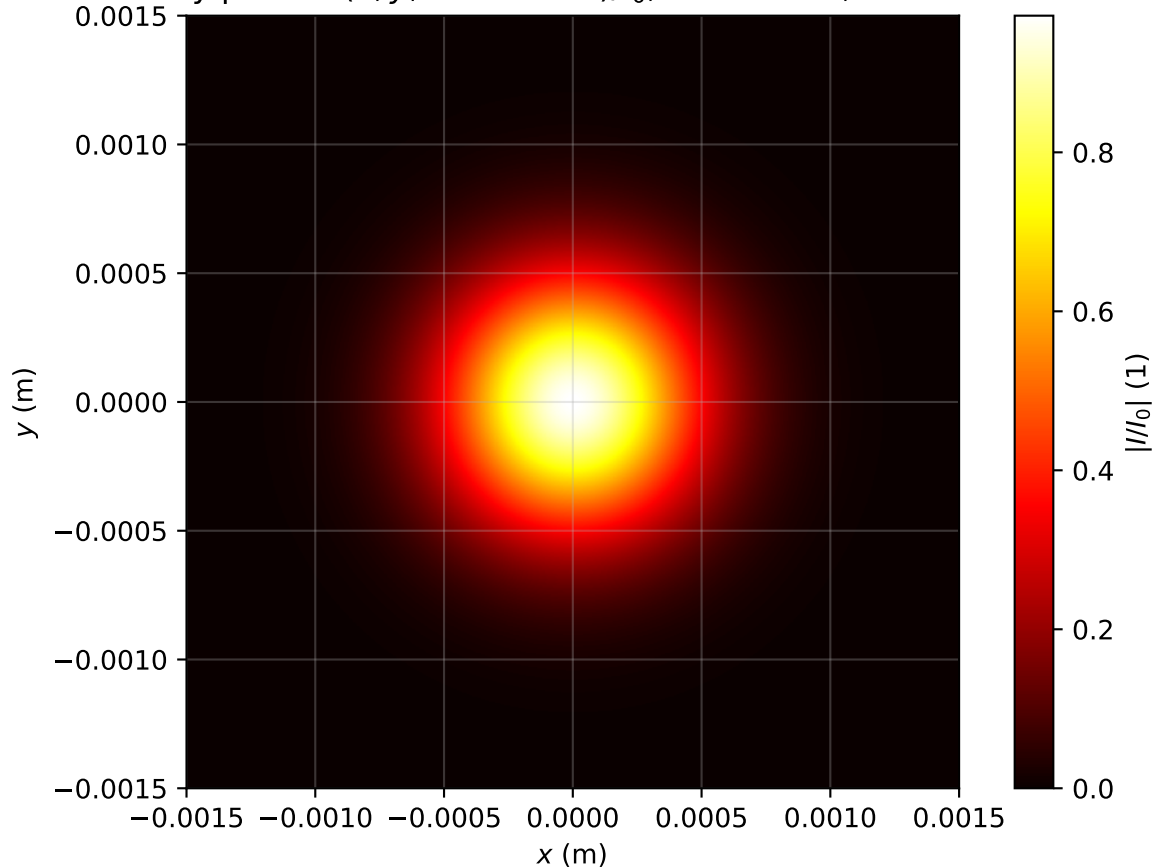
Intensity profile I(x, y, z = 0.557m)/I_0 , Pin=0.2Pcr, artificial time
